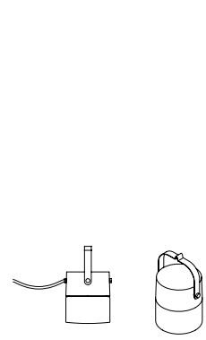
ARTICLE 1010 DIMENSIONS glass Ø 130 h 220 1,5 mt cable POWER 1 x E27 max 25W
