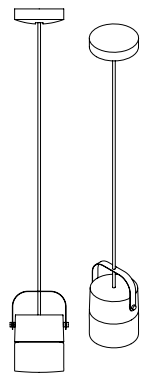
ARTICLE 1010S DIMENSIONS base Ø 130 glass Ø 130 h 250 tot.h.max 1500 POWER 1 x E27 max 25W
